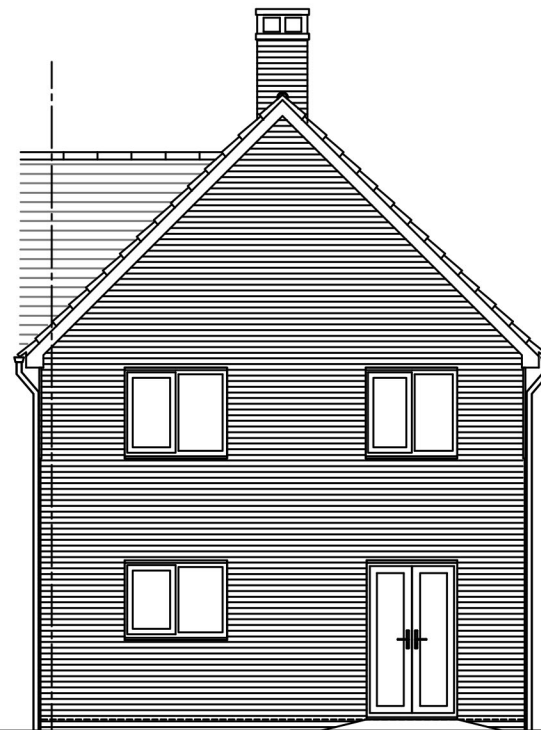
Rear Elevation
